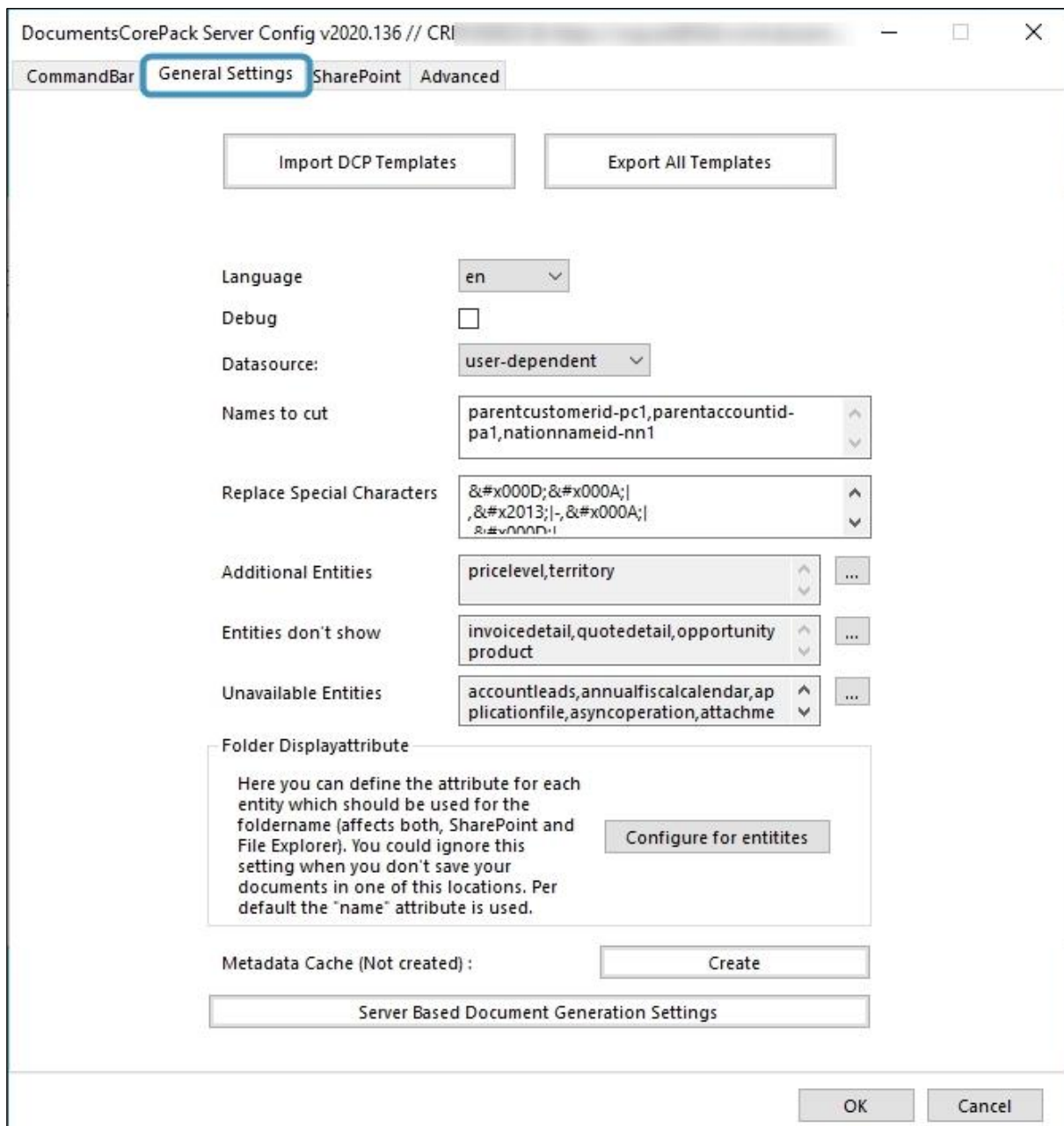
Figure 38: General Settings
